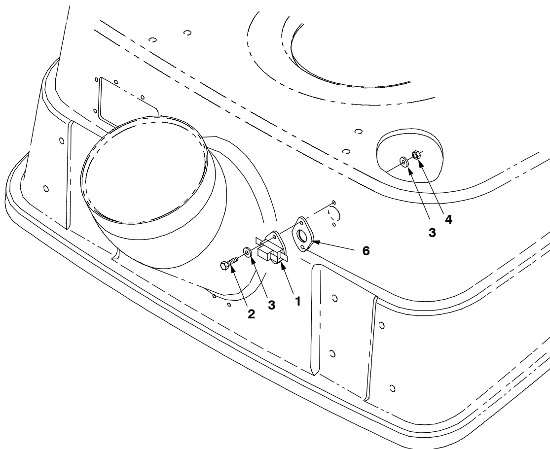
FIG. 2 - Hopper Cover And Thermo-Sentry Assembly
