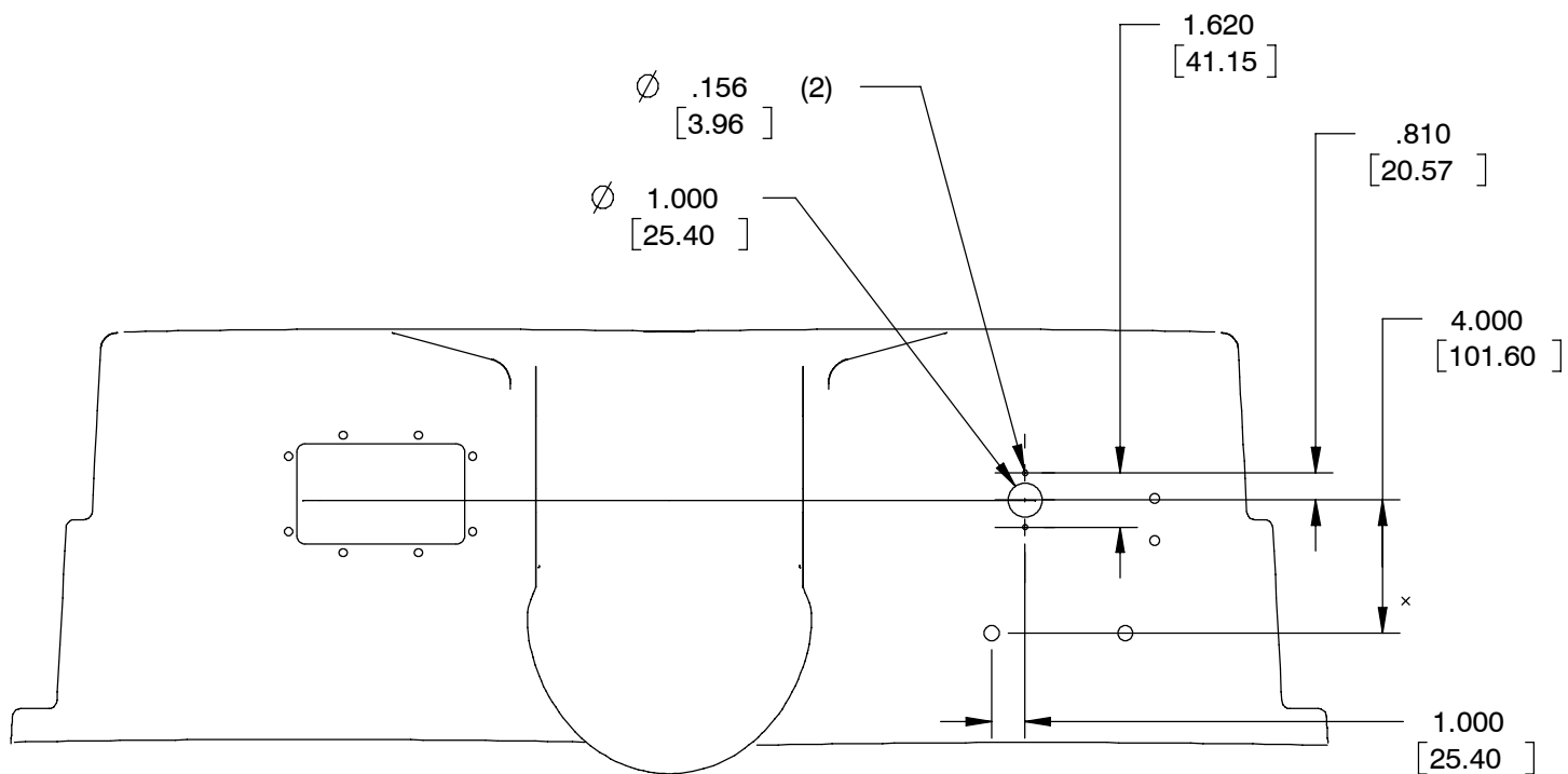
FIG. 1 - Hole Location For Thermo Sentry
